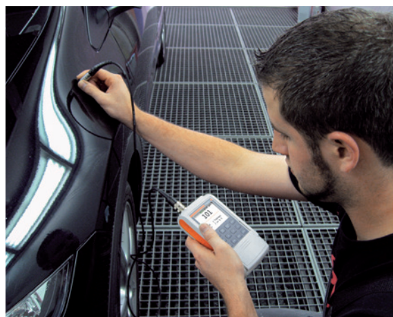
Paint coating thickness measurement using the dual probe FD13H
